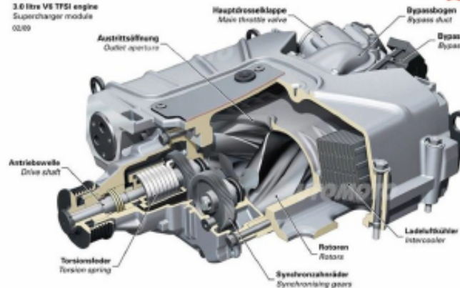
3,0 Liter-V6-TFSI-Motor
